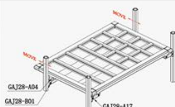
Pallet vertical assembly
